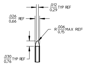
DETAIL Y SCALE 5:1 SEE NOTE 11
