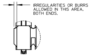
DETAIL Z SCALE 5:1
