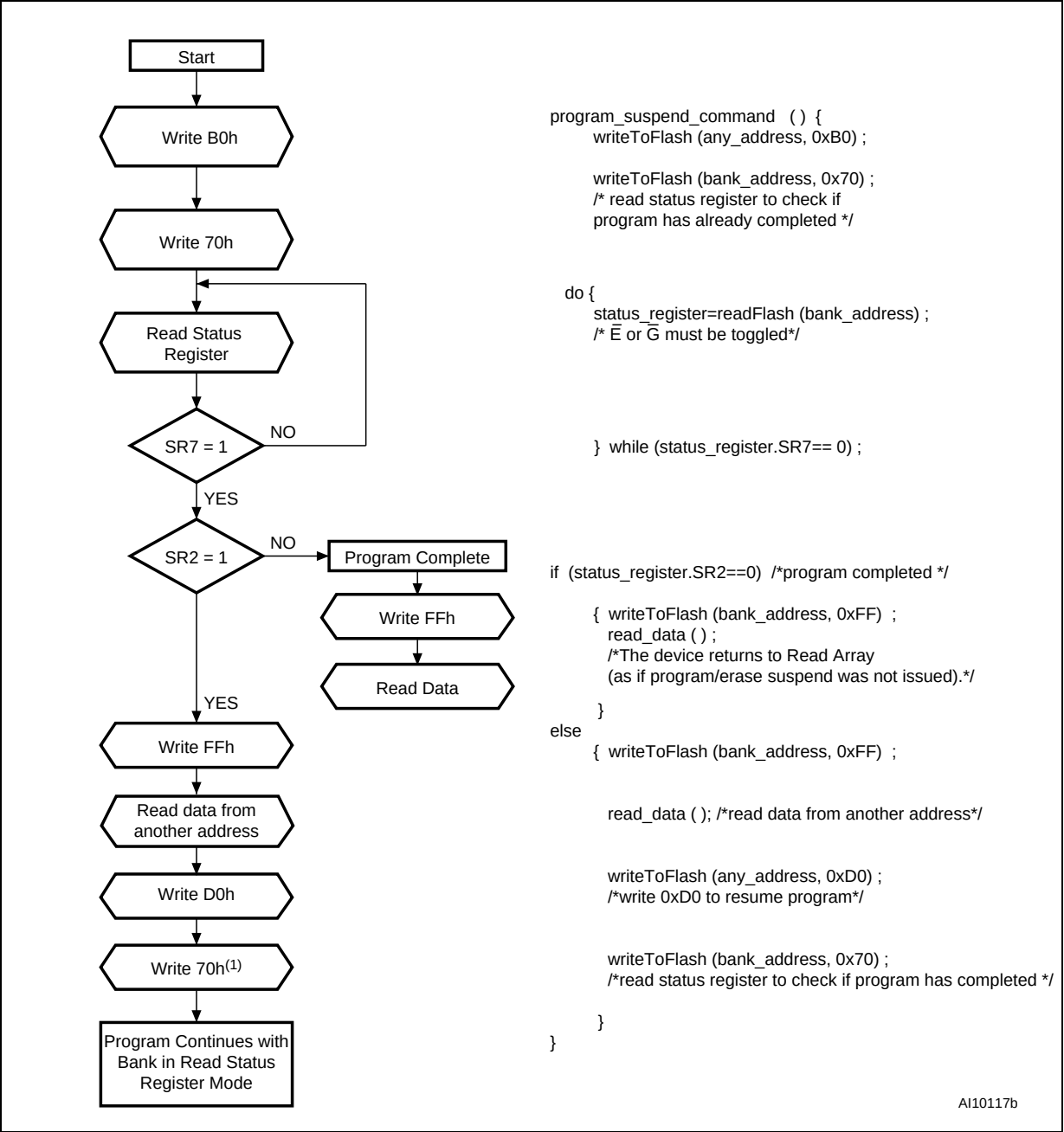
Figure 22. Program suspend and resume flowchart and pseudocode
