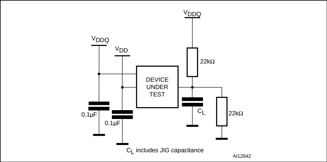
Figure 8. AC measurement load circuit
