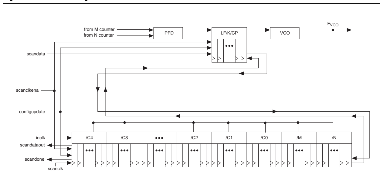
Figure 5-22. PLL Reconfiguration Scan Chain
