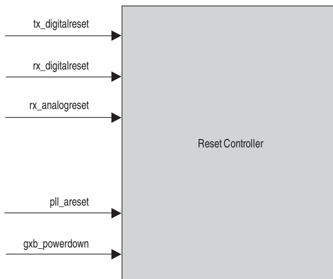
Figure 2-1. Reset Control and Power-Down Block
