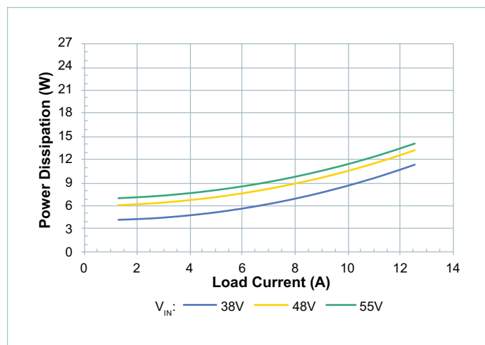
Figure 7 — Power dissipation at T_{CASE} = 25^{\circ}\text{C}
