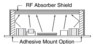
Adhesive Mount Option
