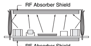
PCB Shield effectiveness can be further enhanced by adding RF absorber material under PCB (see pages 30-34).
