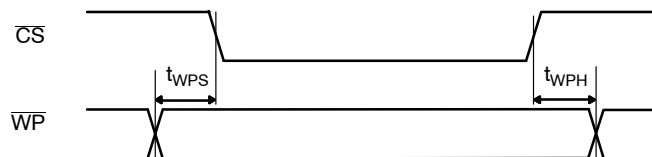
Figure 36. Status Register Write Timing
