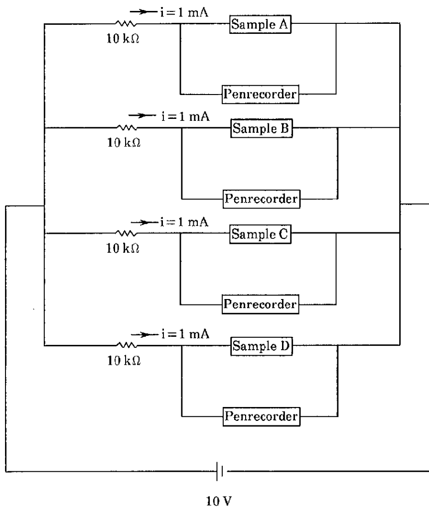
Fig.7 回路抵抗試験 / Circuite Monitering Resistance
