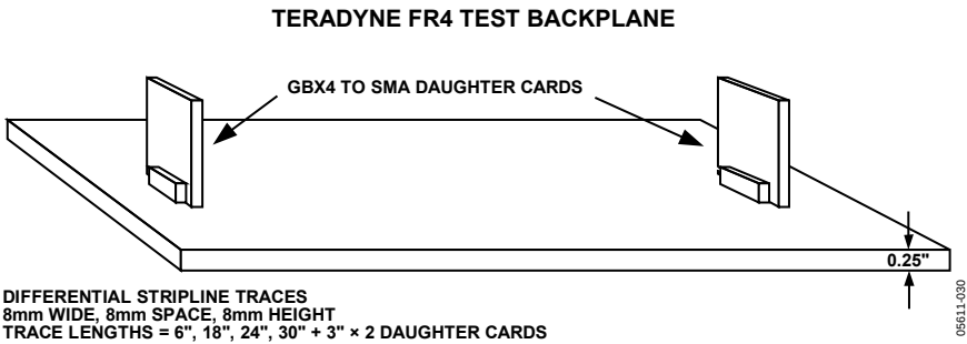
Figure 30. Test Backplane
