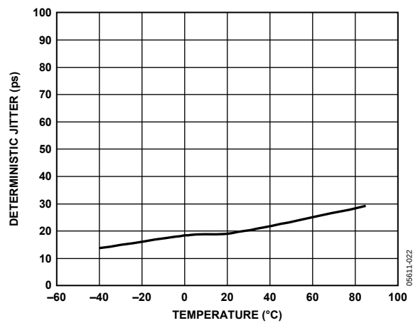
Figure 27. Deterministic Jitter vs. Temperature
