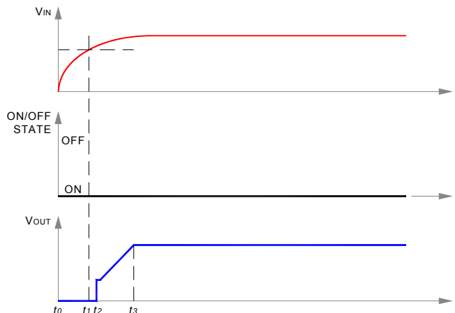
Fig. 7: Start-up scenario #1.
