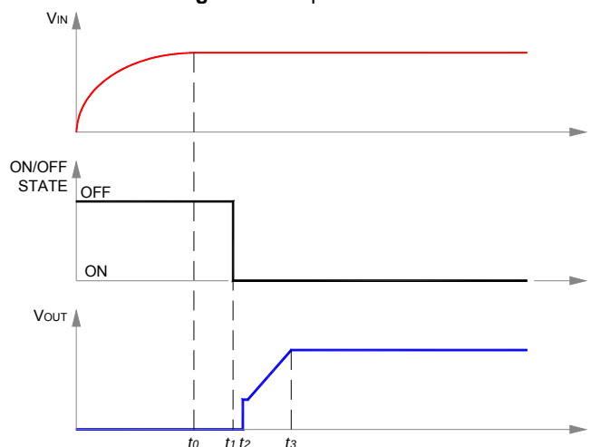
Fig. 8: Start-up scenario #2.
