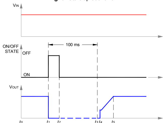
Fig. 9: Start-up scenario #3.
