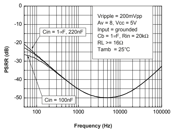
Figure 94. PSRR vs. input capacitor
