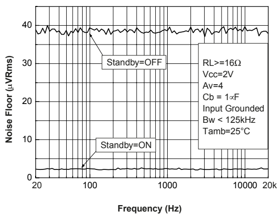
Figure 71. Noise floor V_{CC} = 2V
