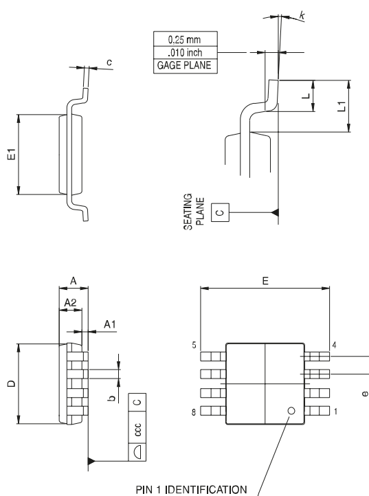
Figure 99. MiniSO-8 drawing
