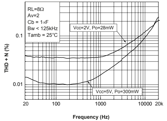
Figure 44. THD + N vs. frequency R_L = 8\ \Omega
