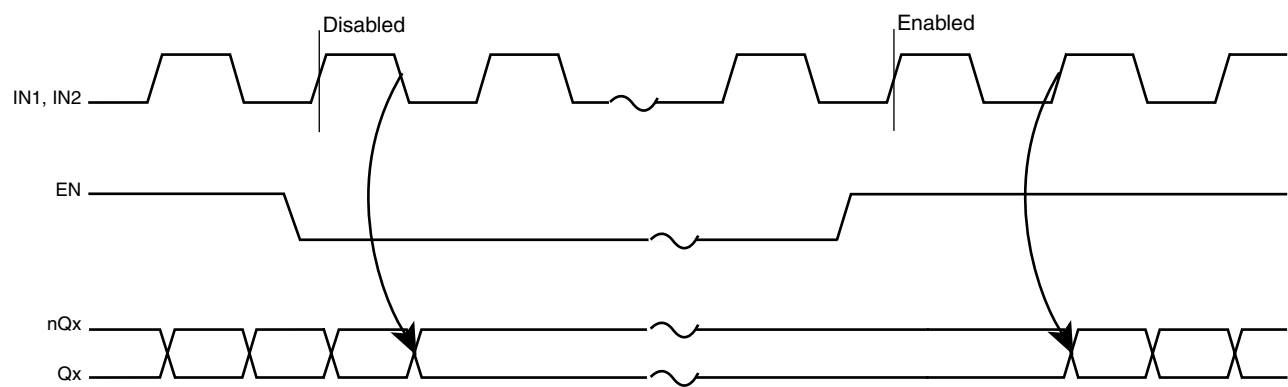
Figure 1. EN Timing Diagram
