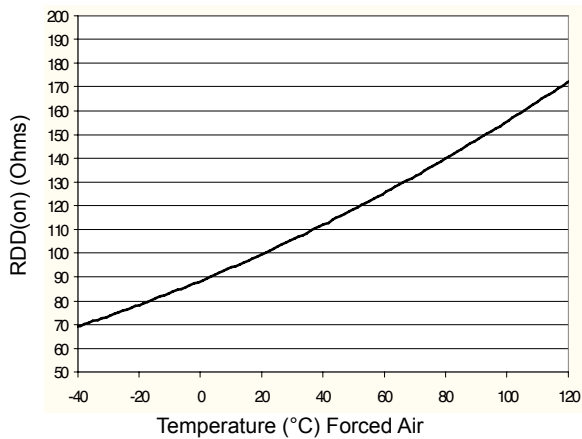
Figure 3. Typical On-Resistance
