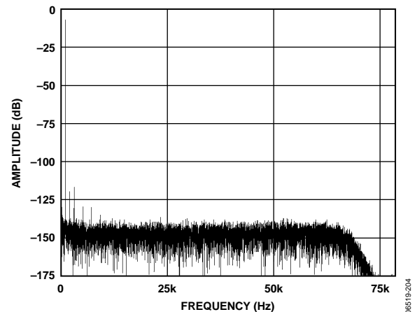
Figure 11. Low Power Mode; FFT, 1 kHz, -6 dB Input Tone, 128× Decimation Rate
