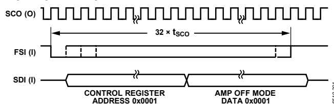
Figure 34. Writing to the AD7765 Control Register Turning Off the On-Board Differential Amplifier
