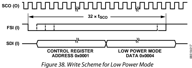
Figure 38. Write Scheme for Low Power Mode
