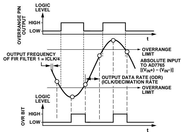
Figure 37. OVERRANGE Pin and OVR Bit vs. Absolute Voltage Applied to the Modulator
