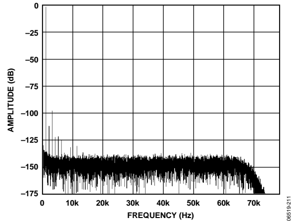
Figure 9. Low Power Mode; FFT, 1 kHz, -0.5 dB Input Tone, 128× Decimation Rate
