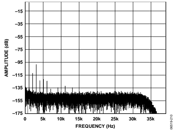
Figure 10. Low Power Mode; FFT, 1 kHz, -0.5 dB Input Tone, 256× Decimation Rate
