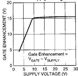
Gate Enhancement vs. Supply Voltage
