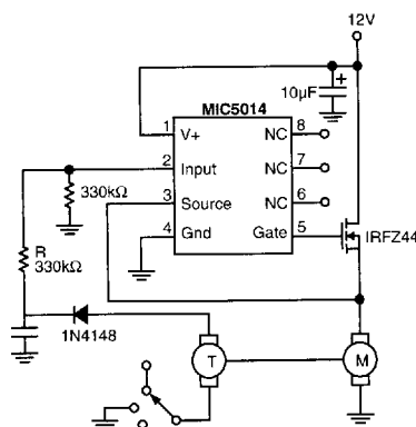
Figure 10. Motor Stall Shutdown
