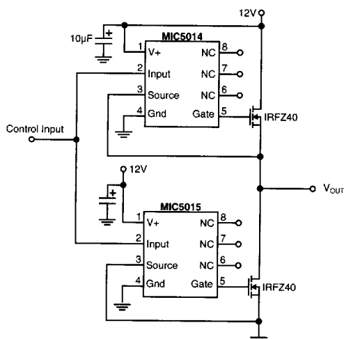
Figure 13: Push-Pull Driver
