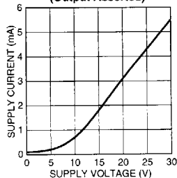
Supply Current (Output Asserted)
