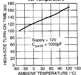
High-Side Turn-On Time vs. Temperature
