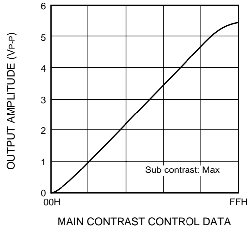
MAIN CONTRAST CONTROL CHARACTERISTICS
