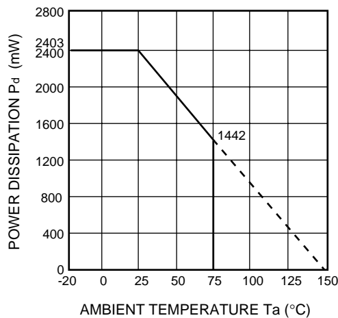
THERMAL DERATING
