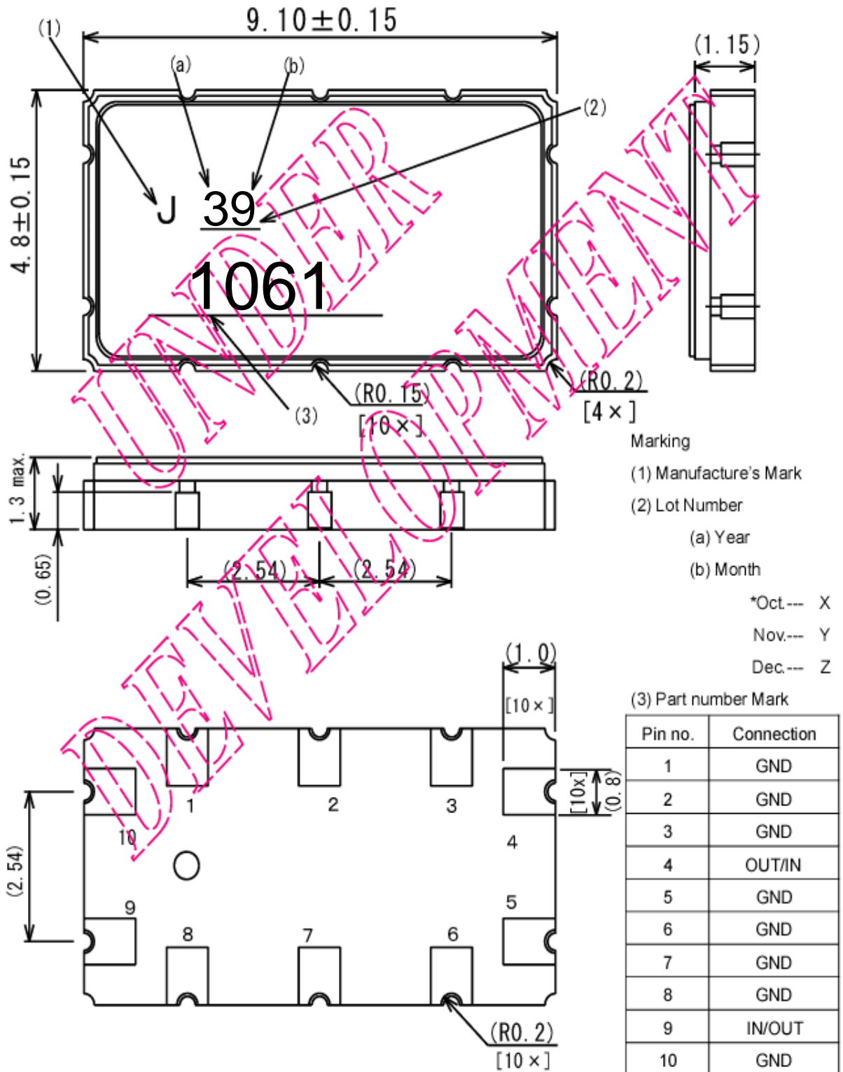
Fig.2 Package dimensions (in mm)
