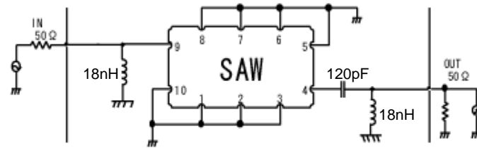
Fig.1 Measuring circuit
