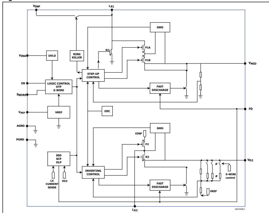
Figure 2. Block schematic
