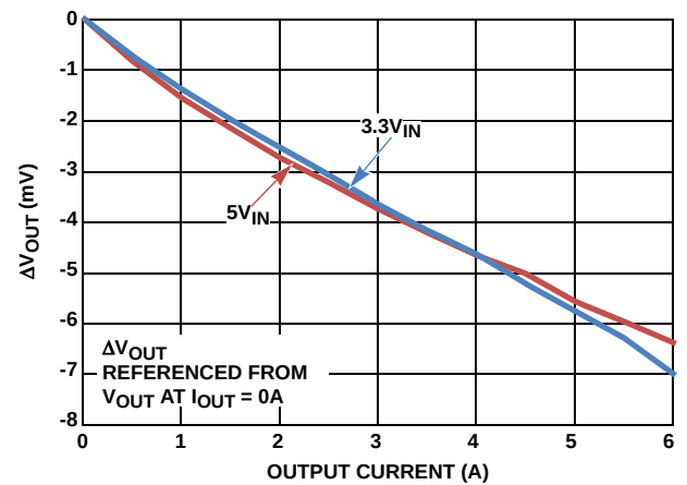
FIGURE 40. LOAD REGULATION, V_{OUT} = 1.8\text{V} , T_A = +25^\circ\text{C}
