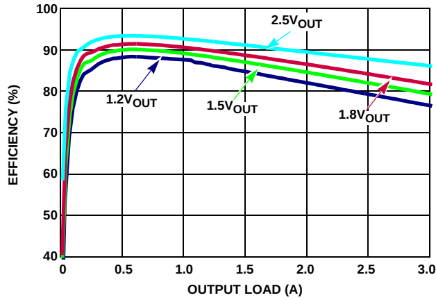
FIGURE 5. EFFICIENCY, V_{IN} = 3.3\text{V} , T_A = +25^\circ\text{C}
