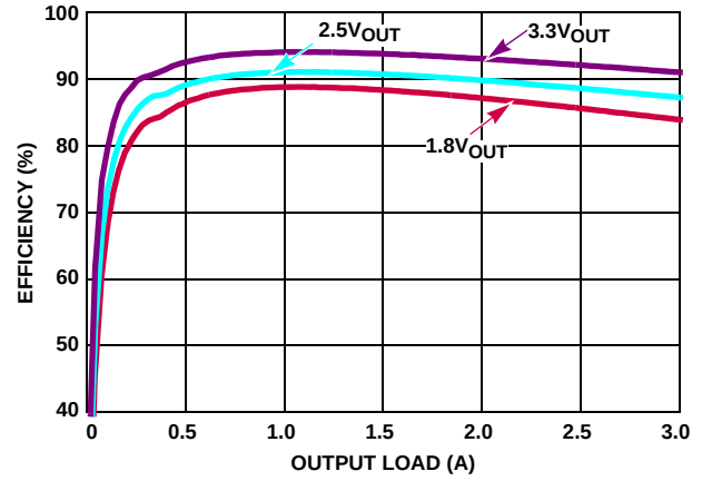
FIGURE 6. EFFICIENCY, V_{IN} = 5\text{V} , T_A = +25^\circ\text{C}
