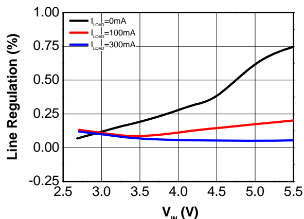
Figure 5. Line Regulation V_{IN} is 2.7 V to 5.5 V and V_{OUT} is 1.8 V, T_A = 25^\circ\text{C}
