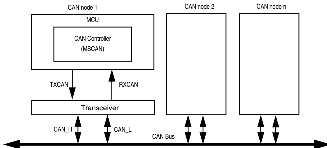
Figure 12-3. CAN System
