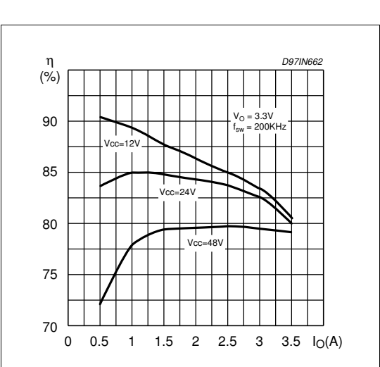
Figure 28. Efficiency vs. output current (see Figure 5 )
