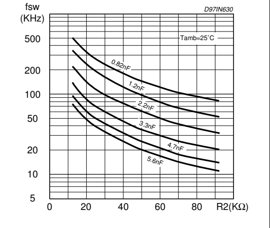
Figure 17. Switching frequency vs. R_2 and C_7
