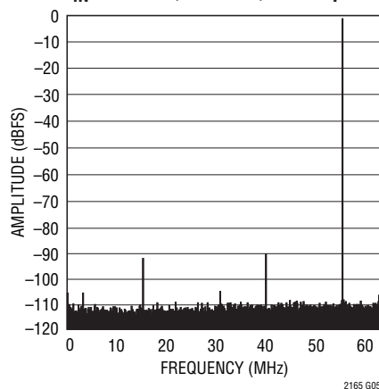
LTC2165 64k Point FFT, f_{IN} = 70\text{MHz} , -1dBFS, 125Msps
