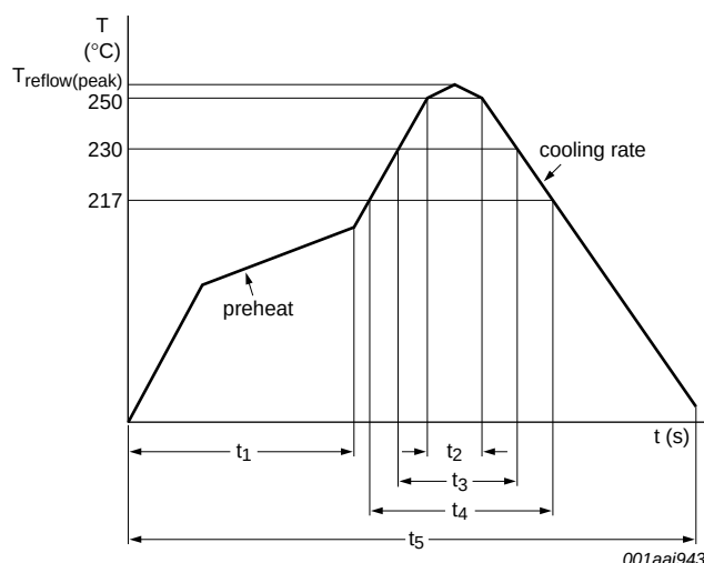
Fig 22. Pb-free solder reflow profile
