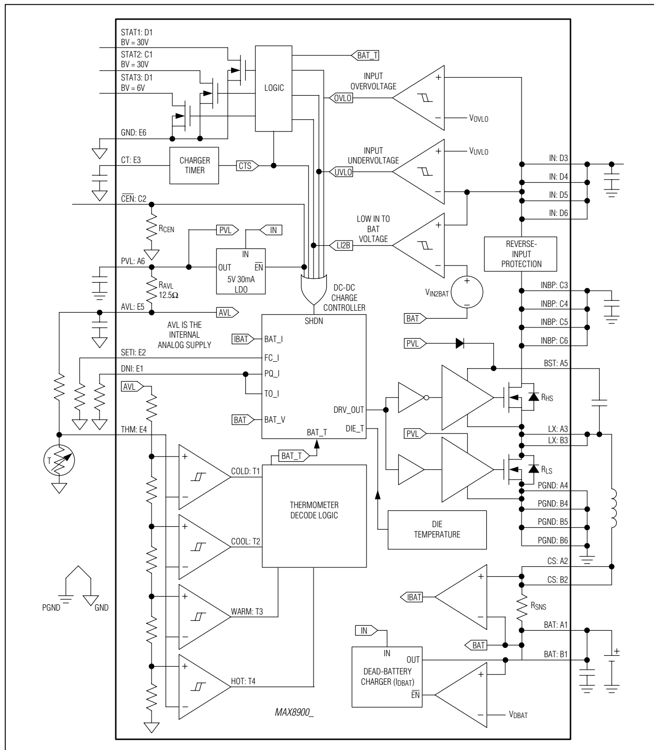
Figure 3. Functional Diagram
