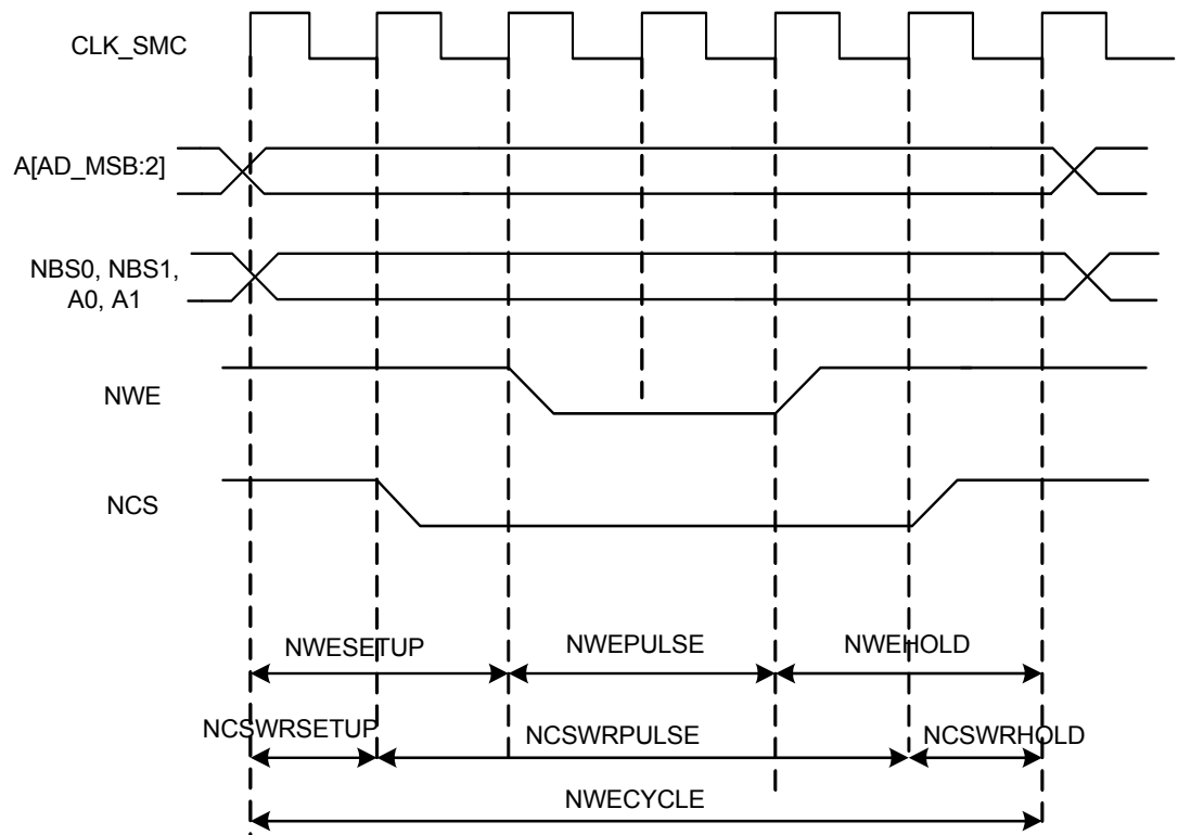
Figure 15-11. Write Cycle
