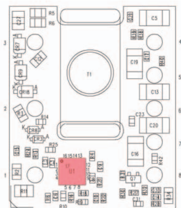
Figure 4. Thermal Shutdown
