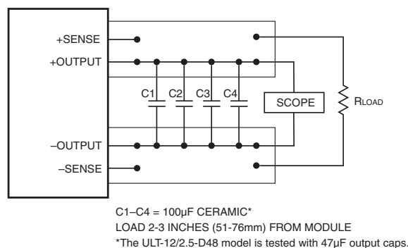
Figure 3. Measuring Output Ripple/Noise (PARD)
