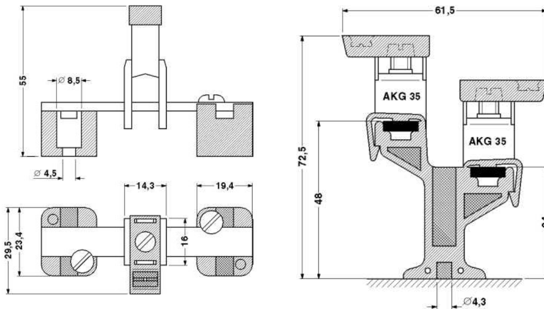
Dimensioned drawing
