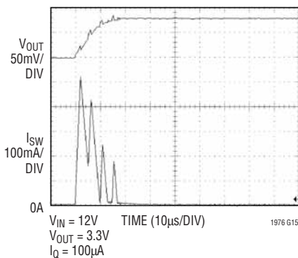
LT1976 Burst Mode Operation
