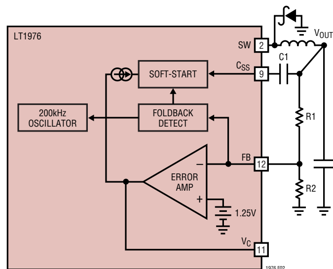
Figure 2. Feedback Network
