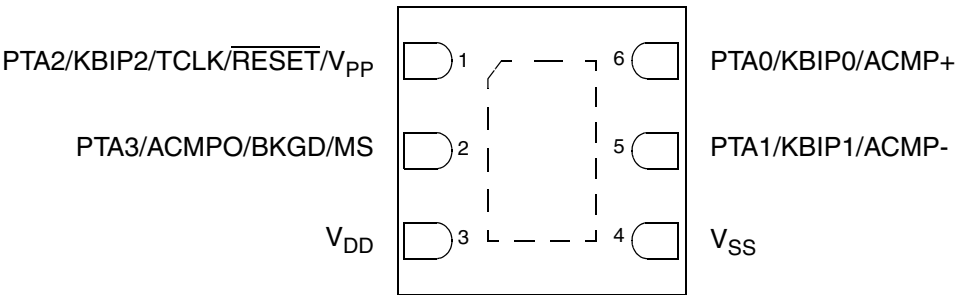
Figure 2-1. MC9RS08KA2 Series in 6-Pin DFN
