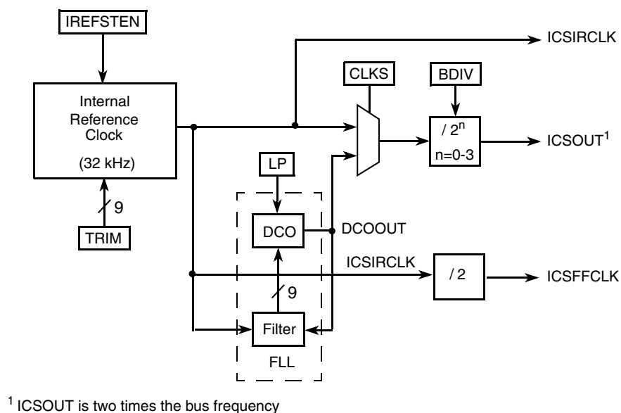
Figure 9-2. Internal Clock Source (ICS) Block Diagram
