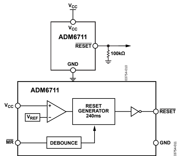
Figure 10. Ensuring a Valid RESET Output Down to V_{\text{CC}} = 0 \text{ V}
