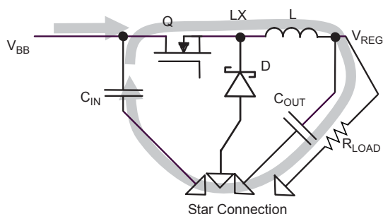
Figure 5. FET on-cycle current conduction paths
