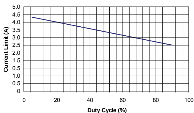
Figure 3. Current limit versus duty cycle
