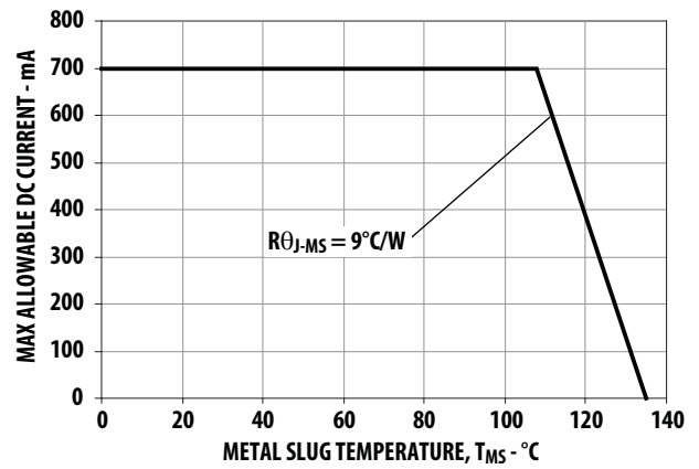
Figure 10. Maximum Forward Current vs. Metal Slug Temperature. Derated based on T_{JMAX} = 125^\circ\text{C} , R_{\theta MS} = 9^\circ\text{C/W}
