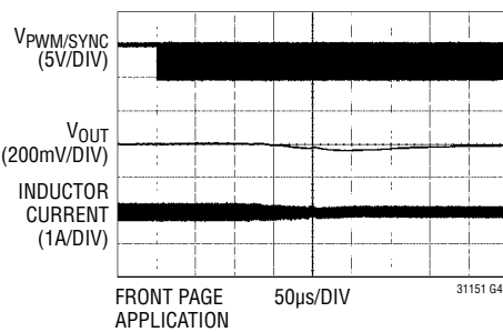
Phase-Locked Loop Acquisition, V_{IN} = 24\text{V} , 1.2MHz Clock
