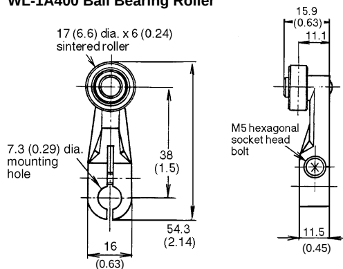
WL-1A400 Ball Bearing Roller
