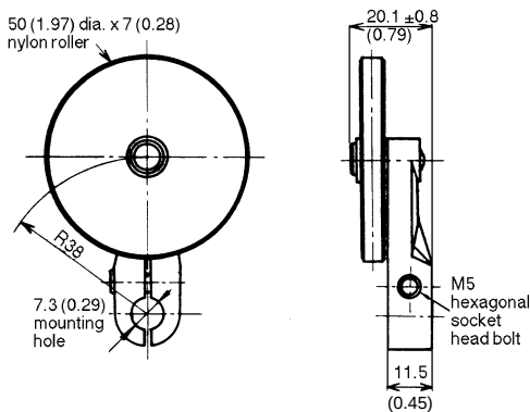
WL-1A106 Nylon Back Mount Roller
