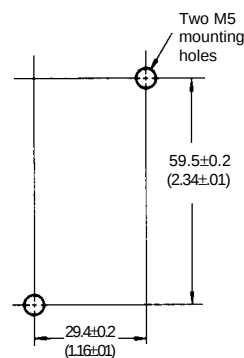
Mounting holes
