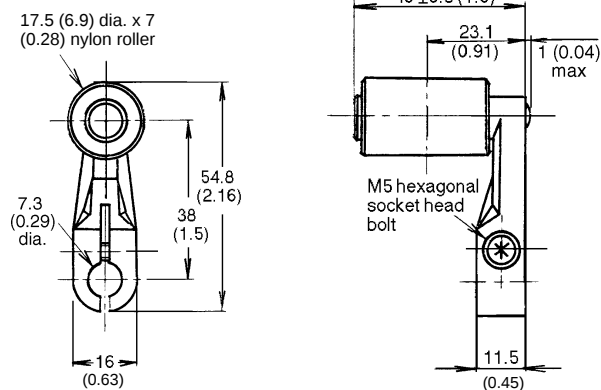
WL-1A104 Nylon Roller
