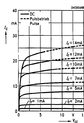
Figure 10. Output Characteristics SFH600-2, -3 ( T_A=25^\circ\text{C} ) I_C=f(V_{CE})
