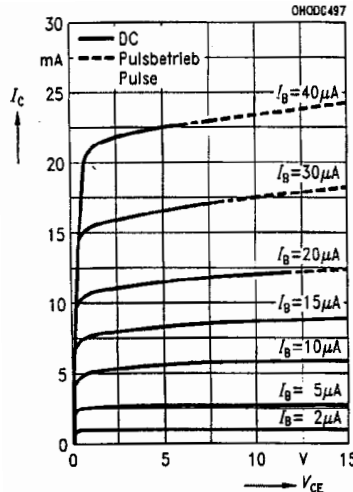
Figure 10. Output Characteristics SFH600-2, -3 ( T_A=25^\circ\text{C} ) I_C=f(V_{CE})
