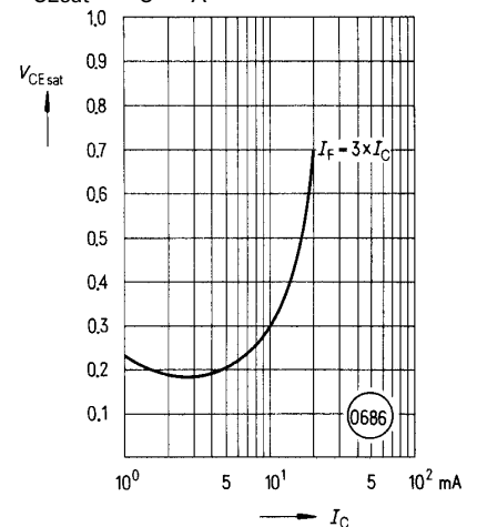
Figure 14. Saturation Voltage versus Collector Current and Modulation Depth SFH600-1 V_{CEsat}=f(I_C) ( T_A=25^\circ\text{C} )
