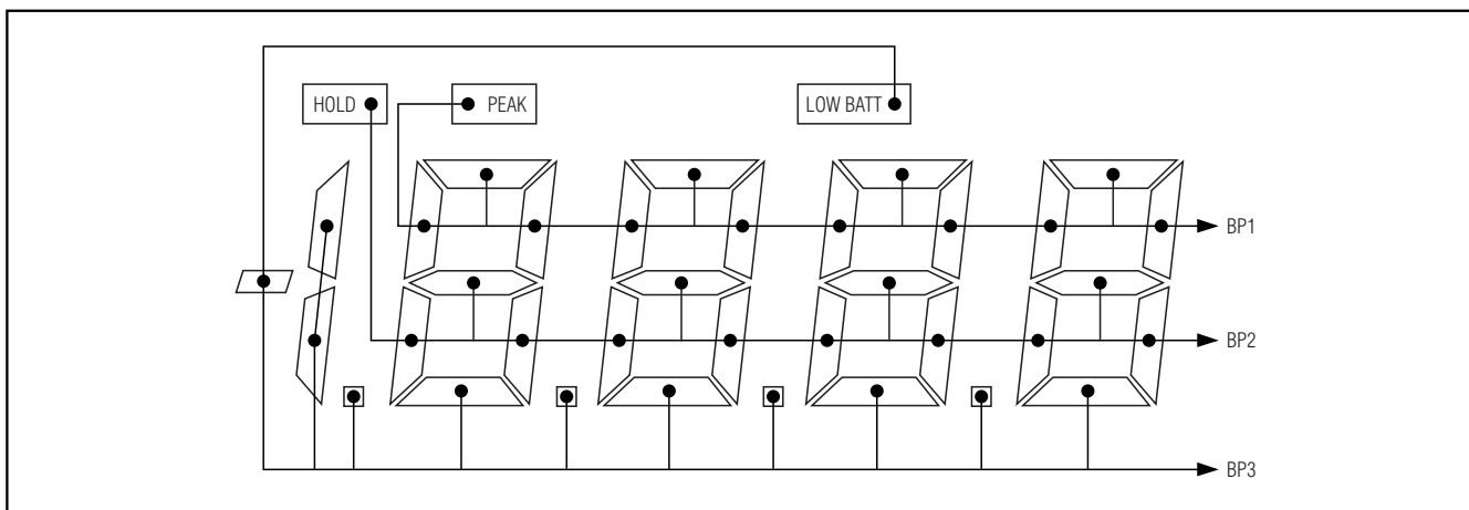
Figure 4. Backplane Connection for the MAX1494 (4.5 Digits)
