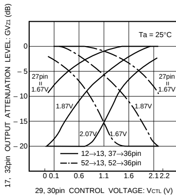
Fig. 5 Zoom control position variation characteristics
