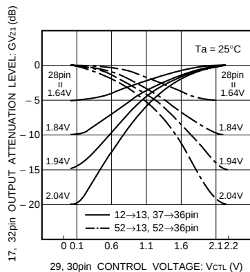
Fig. 4 Zoom control slope variation characteristics
