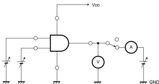
Fig. 1 DC characteristics
