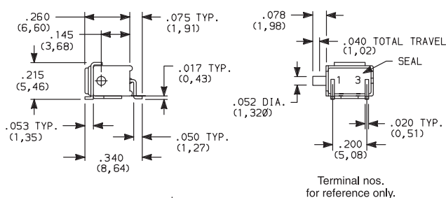
PC MOUNTING
