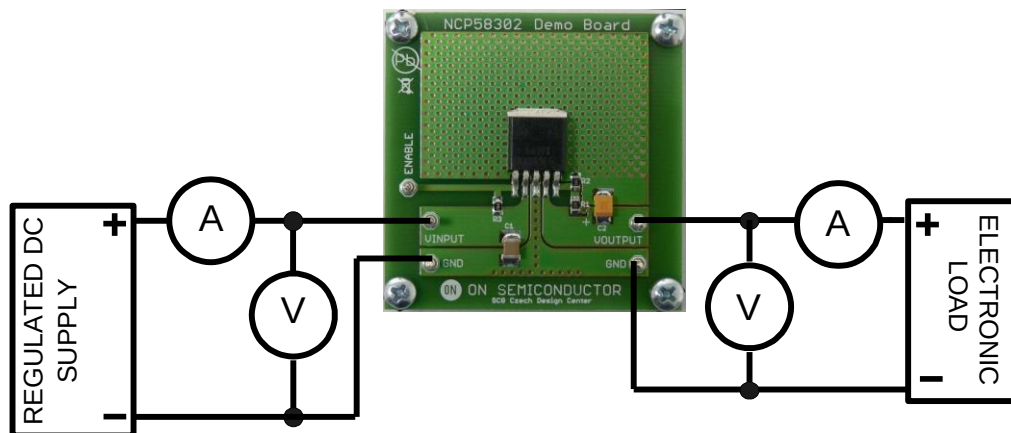
Figure 1: Test Setup
