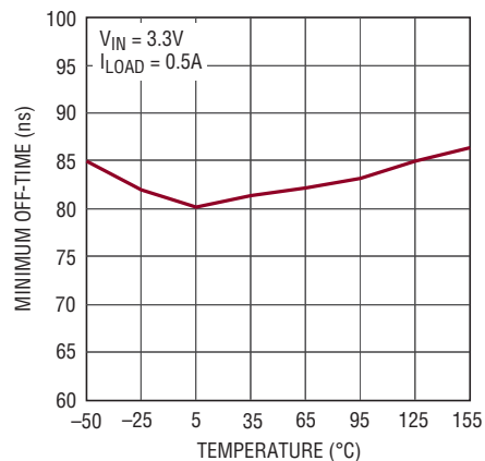
Minimum Off-Time
