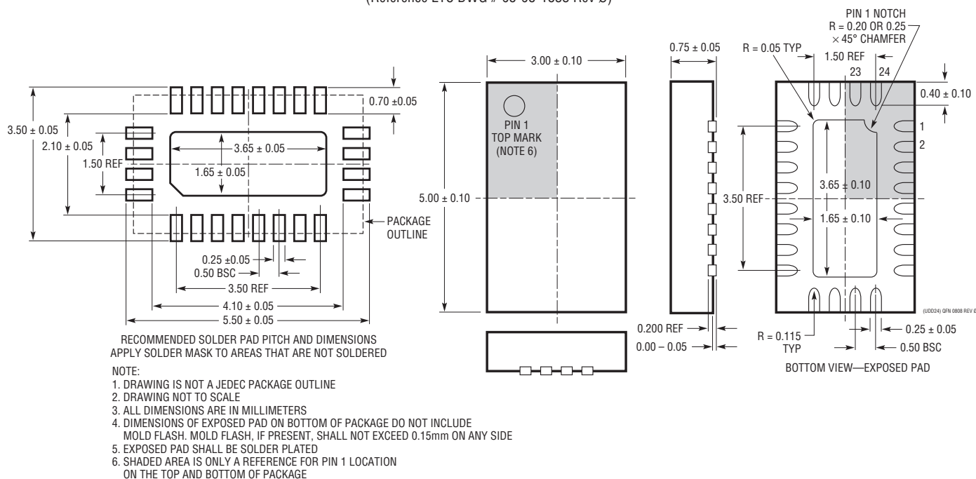
UDD Package 24-Lead Plastic QFN (3mm × 5mm) (Reference LTC DWG # 05-08-1833 Rev 0)
