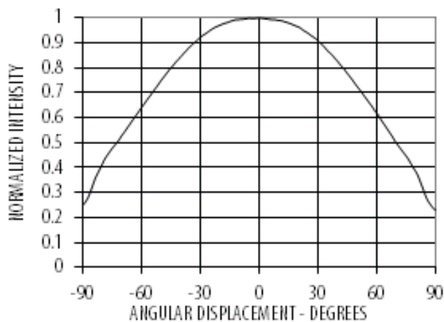
Figure 5 Radiation Pattern
