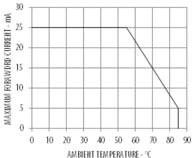
Figure 7 Derating Curve
