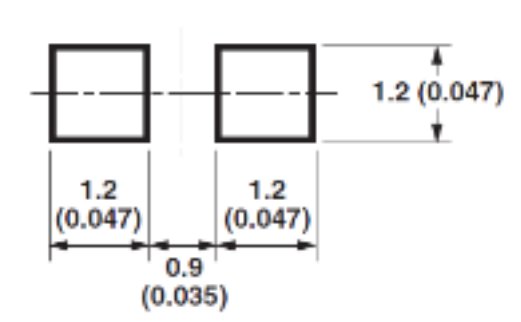
Recommended Soldering Land Pattern
