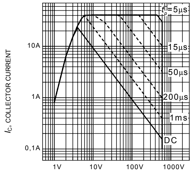
Figure 2. Safe operating area
