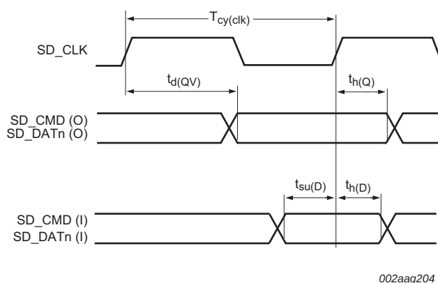
Fig 40. SD/MMC timing
