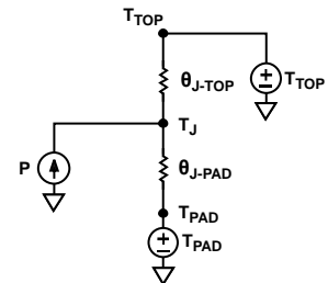
Figure 39. Electrical Model for Thermal Calculations
