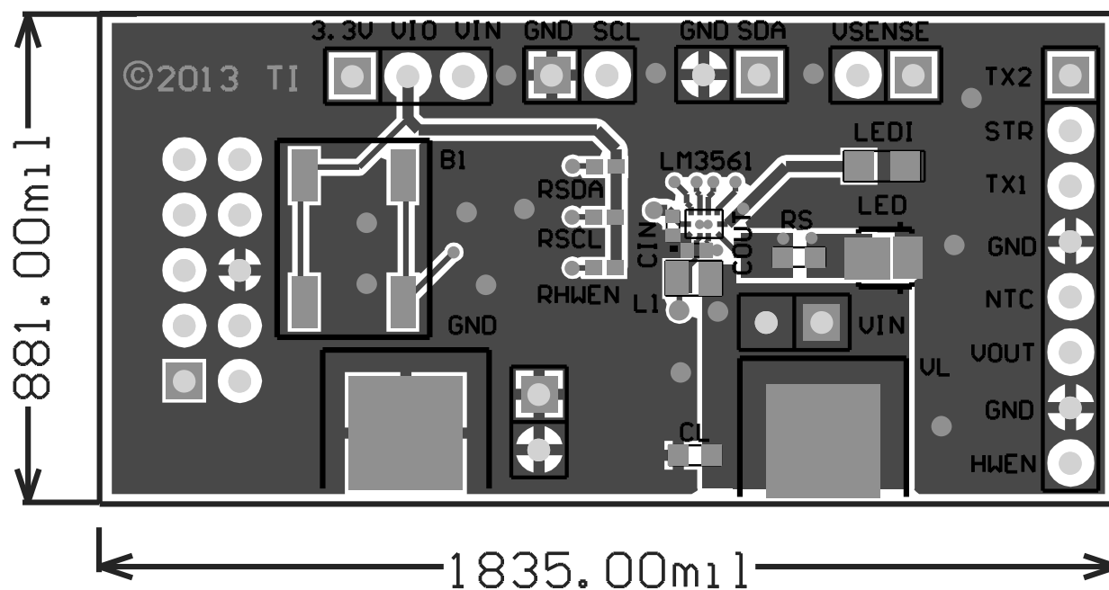
Figure 2. Top Layer
