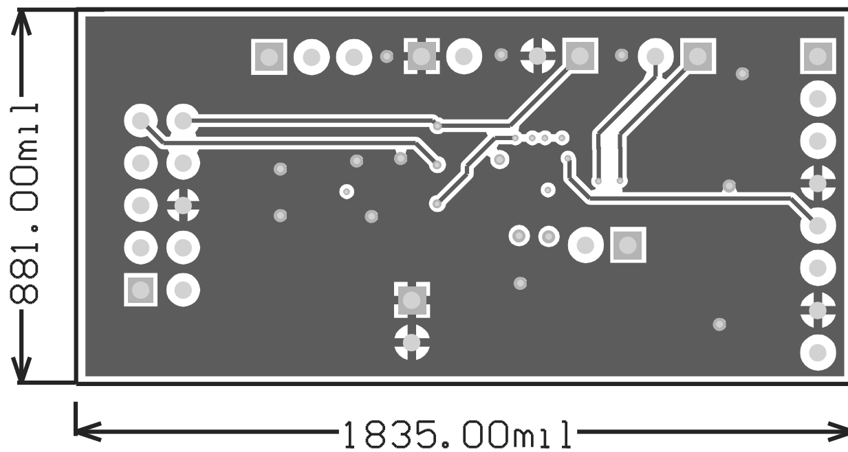
Figure 4. Mid Layer 2
