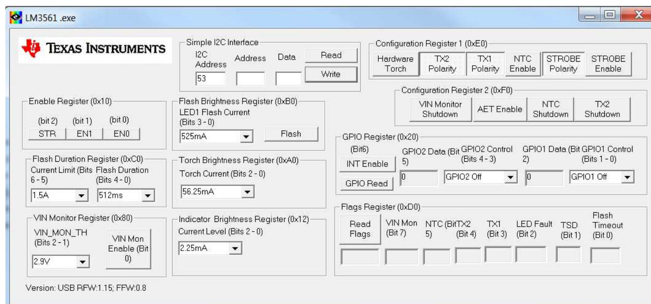
Figure 6. LM3561.exe GUI
