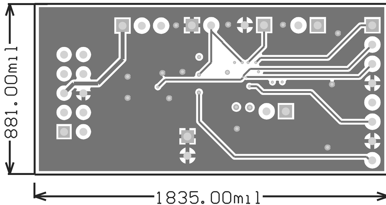
Figure 3. Mid Layer 1
