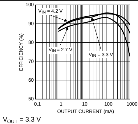
Figure 39. Autocode Efficiency vs I_{LOAD}
