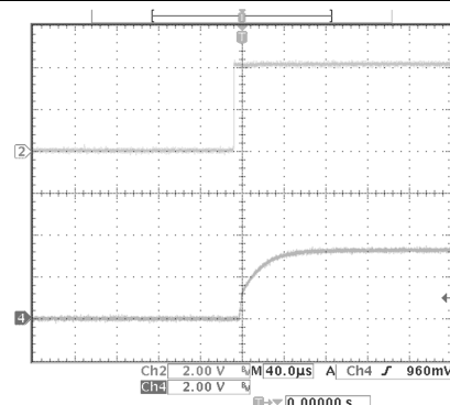
V_{IN} = 0 to 3.6 V V_{OUT} = 3.3 V Load = 1 mA
