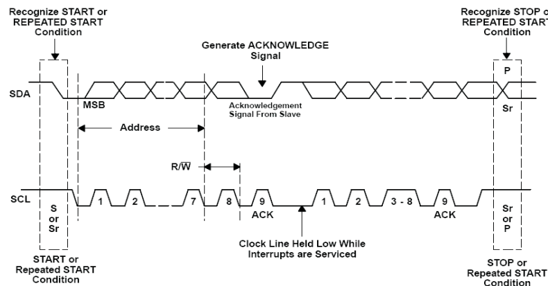
Figure 53. Bus Protocol
