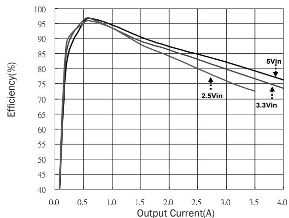
Figure 10. Efficiency(V IN )
