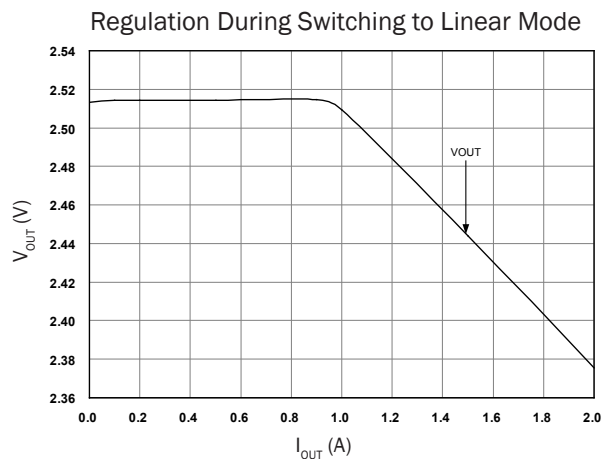
Figure 13. Loading Regulation
