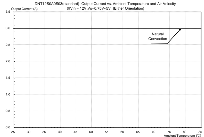
Figure 29: Output current vs. ambient temperature and air velocity @ V_{in}=12V , V_o=0.75V \sim 5.0V (Either Orientation)
