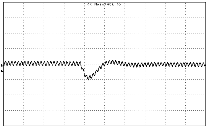
Figure 16: Typical transient response to step load change at 2.5A/μS from 50% to 100% of I_o , max at 12Vin, 5.0V out ( C_{out} = 1\mu F ceramic, 10μF tantalum) (200mV/div, 20uS/div)
