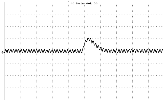
Figure 15: Typical transient response to step load change at 2.5A/μS from 100% to 50% of I_o , max at 12Vin, 5.0V out ( C_{out} = 1\mu F ceramic, 10μF tantalum) (200mV/div, 20uS/div)
