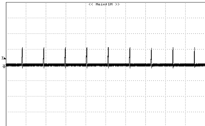
Figure 17: Output short circuit current 12Vin, 0.75Vout (10A/div, 50mS/div)
